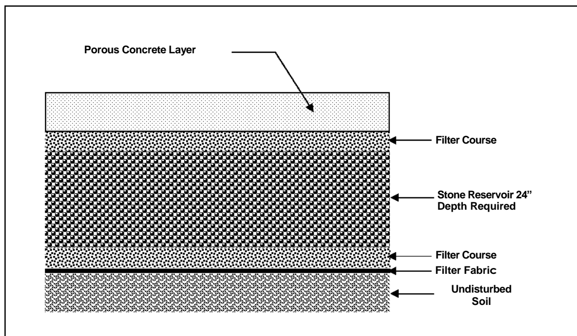
Typical Detail (Source: Georgia SWM Manual)
